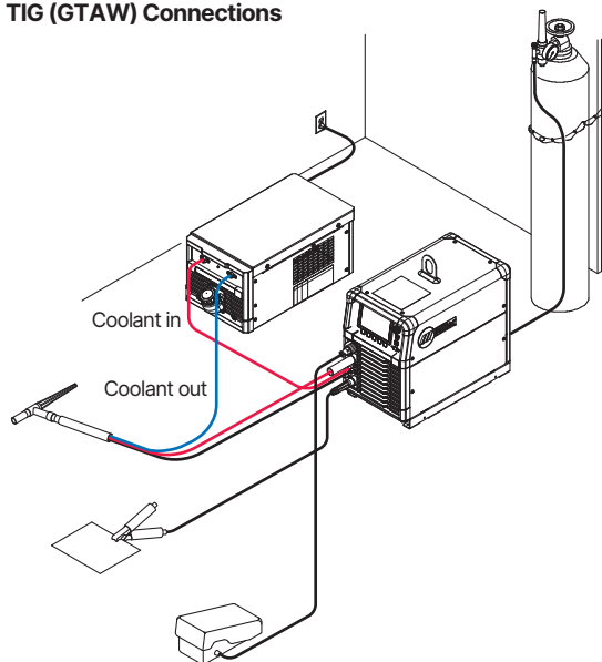
TIG (GTAW) Connections
